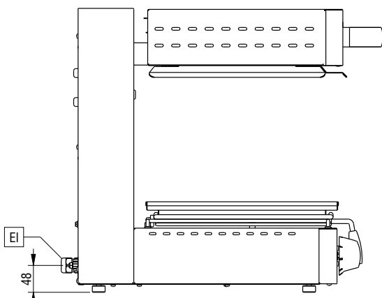
Lateral
